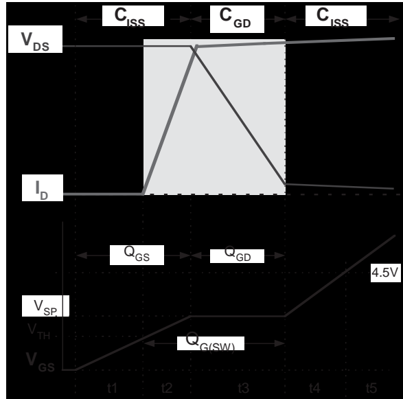
Figure 12. Switching Losses and QG
