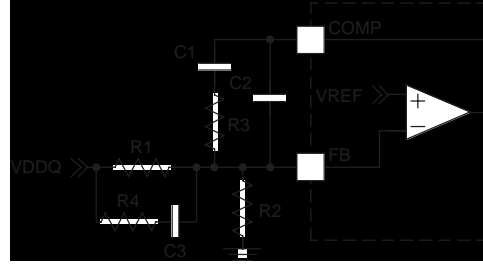
Figure 10. Compensation Network
