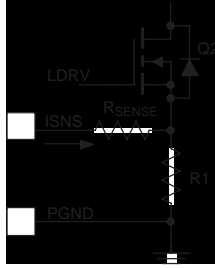
Figure 9. Improving Current Sensing Accuracy
