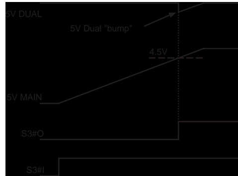
Figure 4. S3 to S0 Transition: 5V DUAL
