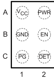
YFP Package 6-Pin DSBGA Top-Through View
