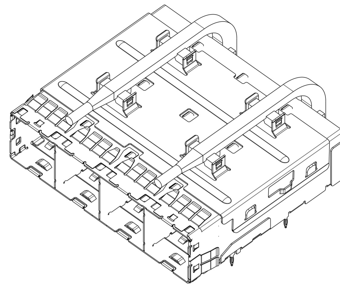
10130603-101LF WITH LIGHT PIPES
