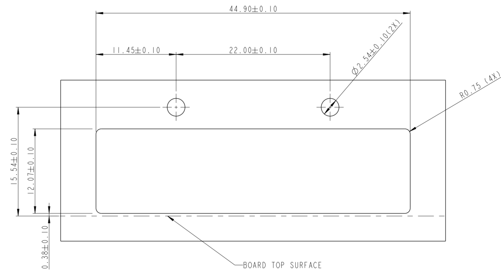
10130603-101LF WITH LIGHT PIPES (LIGHT PIPE SUB-ASSEMBLY WITH MOUNTING CLIP FINAL ASSEMBLY BY CUSTOMER)
