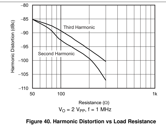
Figure 40. Harmonic Distortion vs Load Resistance
