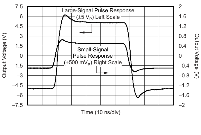
Figure 46. Pulse Response
