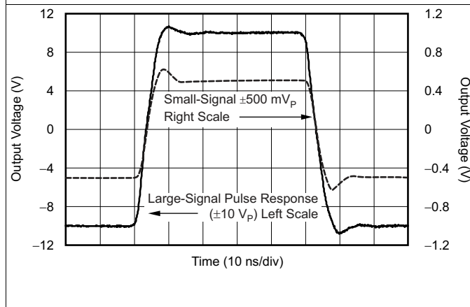
Figure 33. Pulse Response
