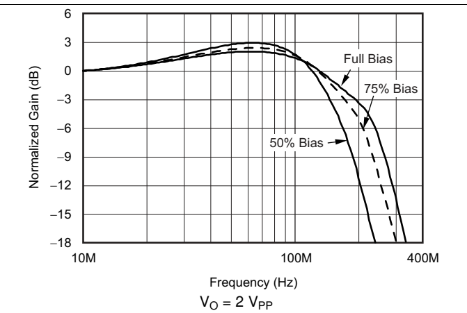
Figure 44. Small-Signal Frequency Response vs Bias
