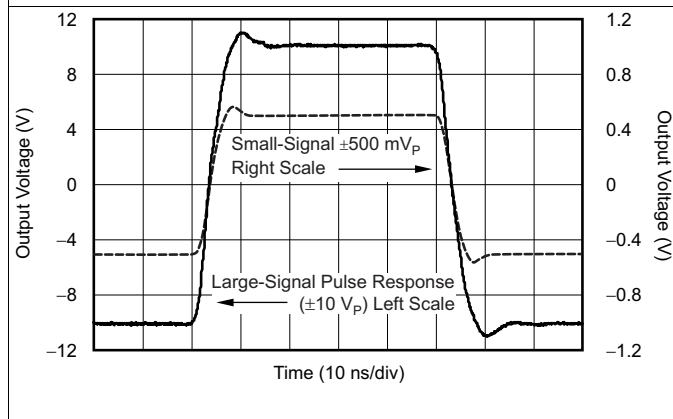
Figure 21. Pulse Response
