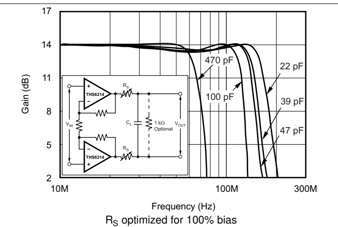
Figure 48. Frequency Response vs Capacitive Load
