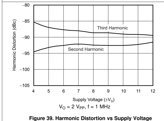
Figure 39. Harmonic Distortion vs Supply Voltage
