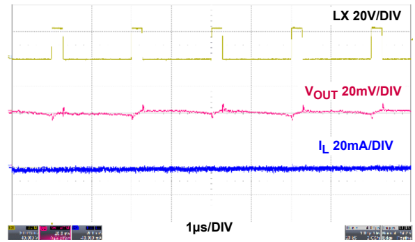
FIGURE 30. STEADY STATE AT NO LOAD, PWM
