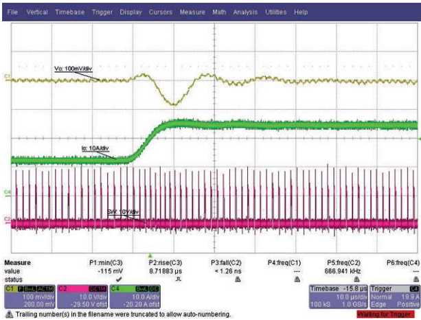
Fig. 28 - Load Step, 12 A to 24 A, 1 A/ \mu\text{s} , t = 10\ \mu\text{s}/\text{div}
