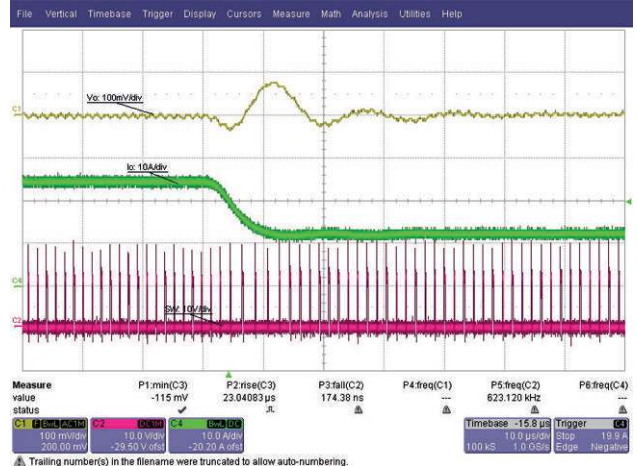
Fig. 31 - Load Release, 24 A to 12 A, 1 A/ \mu\text{s} , t = 10\ \mu\text{s}/\text{div}
