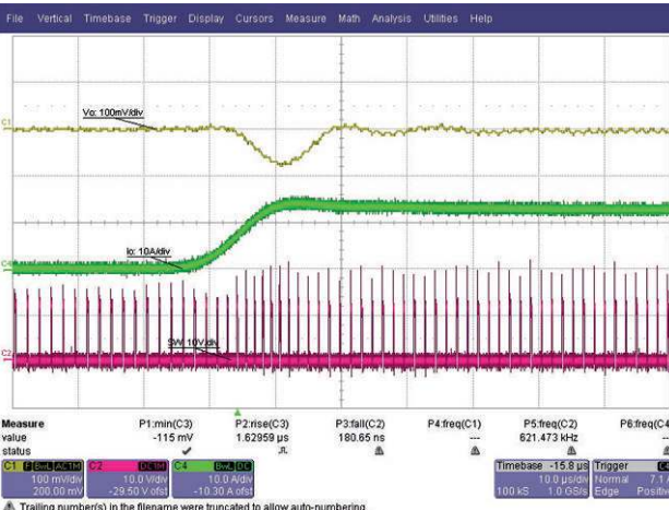
Fig. 30 - Load Step, 0.1 A to 12 A, 1 A/ \mu\text{s} , t = 10\ \mu\text{s}/\text{div} Forced Continuous Conduction Mode
