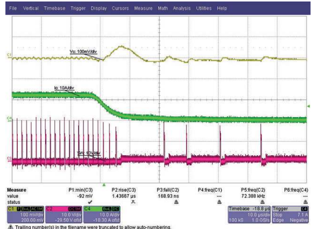
Fig. 32 - Load Release, 12 A to 0.1 A, 1 A/ \mu\text{s} , t = 20\ \mu\text{s}/\text{div} Skip Mode Enabled
