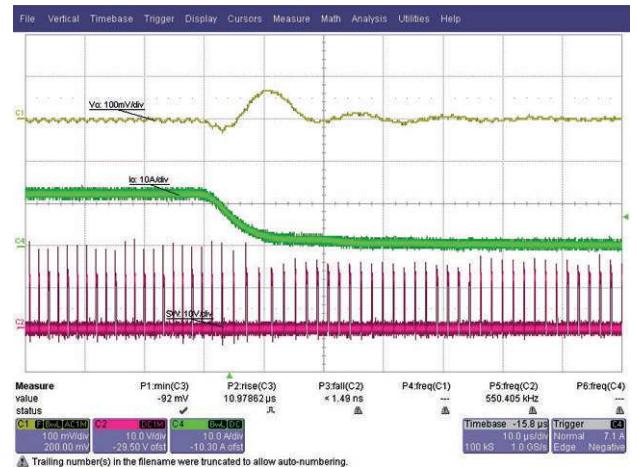
Fig. 33 - Load Release, 12 A to 0.1 A, 1 A/ \mu\text{s} , t = 10\ \mu\text{s}/\text{div} Forced Continuous Conduction Mode
