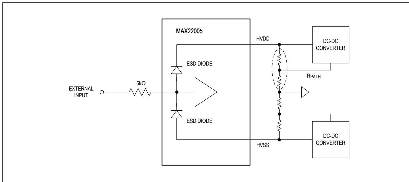
Figure 5. Input Protection
