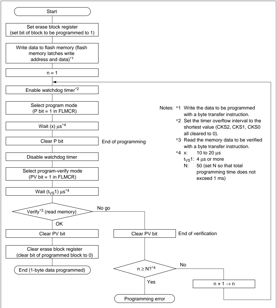
Figure 19.8 Programming Flowchart
