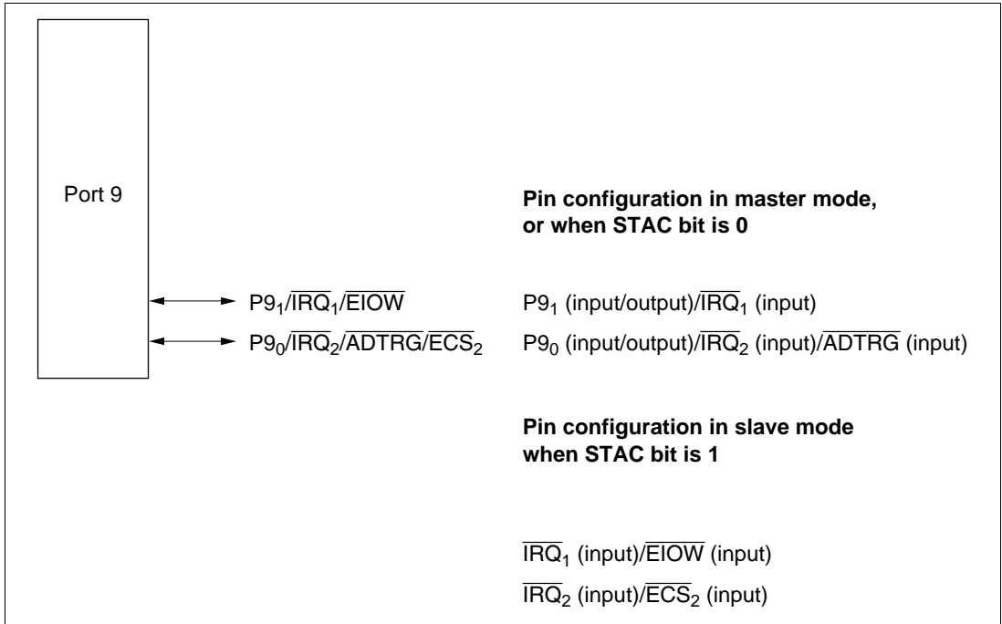
Figure 7.17 Port 9 Pin Configuration (cont)
