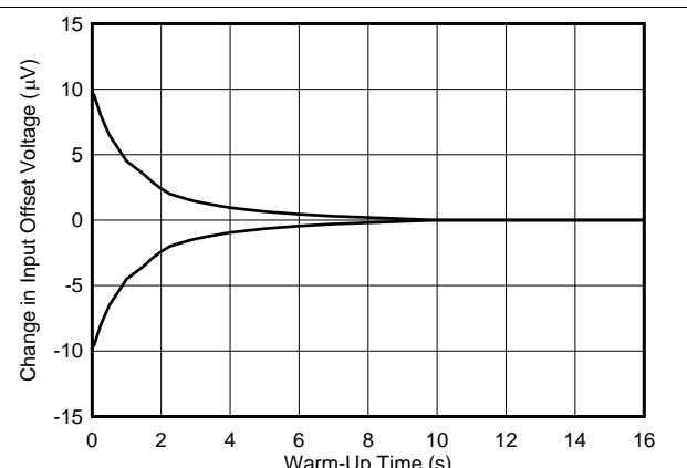
Figure 60. Change in Input Offset Voltage vs Warm-Up Time
