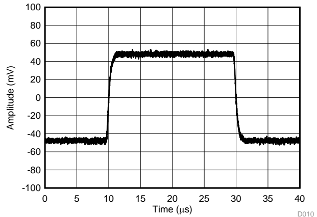
G = 10, R_L = 10\text{ k}\Omega, C_L = 100\text{ pF} Figure 56. Small-Signal Response
