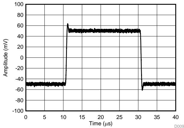
G = 1, R_L = 1\text{ k}\Omega, C_L = 100\text{ pF} Figure 55. Small-Signal Response
