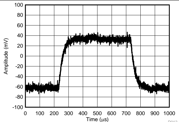
G = 1000, R_L = 10\text{ k}\Omega, C_L = 100\text{ pF} Figure 58. Small-Signal Response
