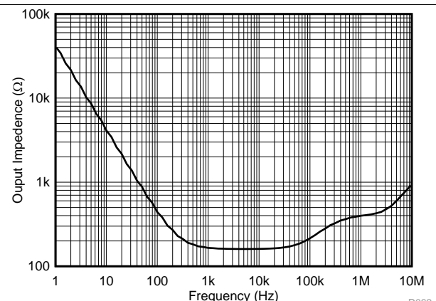
Figure 59. Open-Loop Output Impedance vs Frequency
