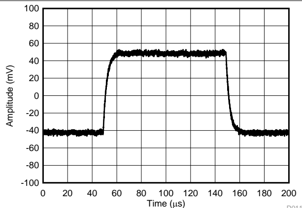
G = 100, R_L = 10\text{ k}\Omega, C_L = 100\text{ pF} Figure 57. Small-Signal Response
