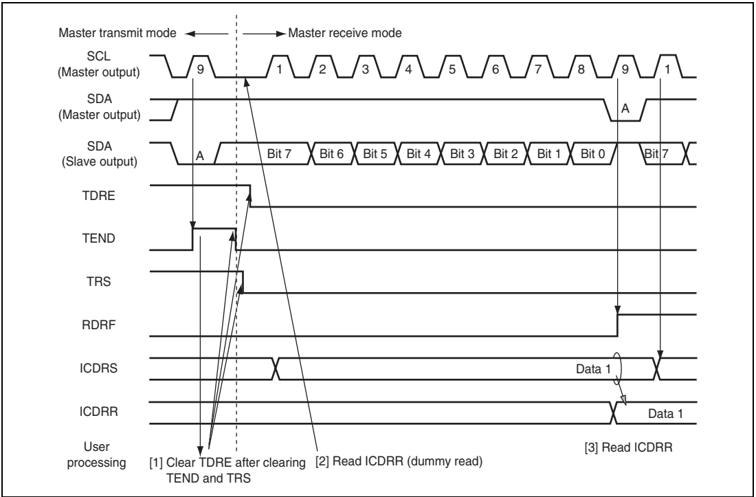
Figure 19.7 Master Receive Mode Operation Timing (1)
