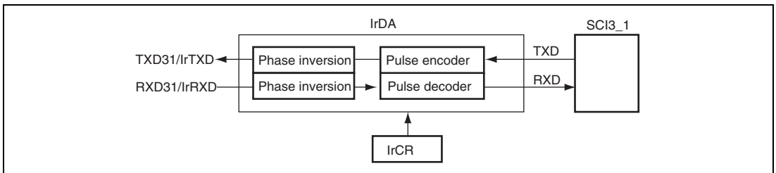
Figure 15.15 IrDA Block Diagram
