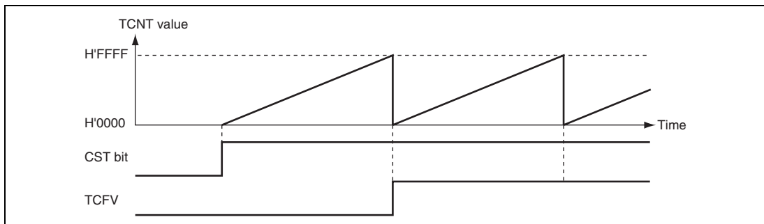
Figure 12.7 Free-Running Counter Operation
