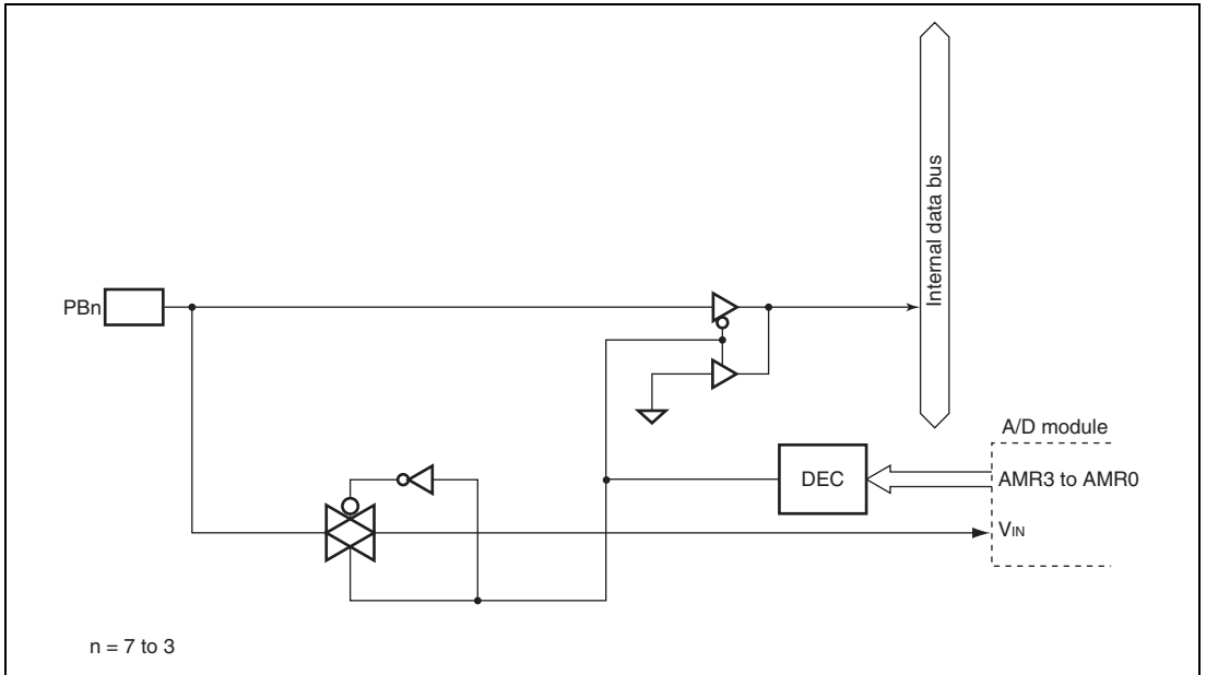
Figure B.10 (a) Port B Block Diagram (PB7 to PB3)
