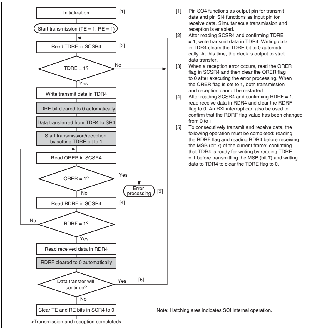
Figure 16.8 Flowchart Example of Simultaneous Transmission and Reception
