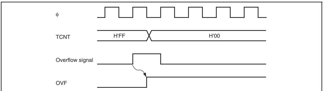
Figure 14.4 Timing of OVF Flag Setting
