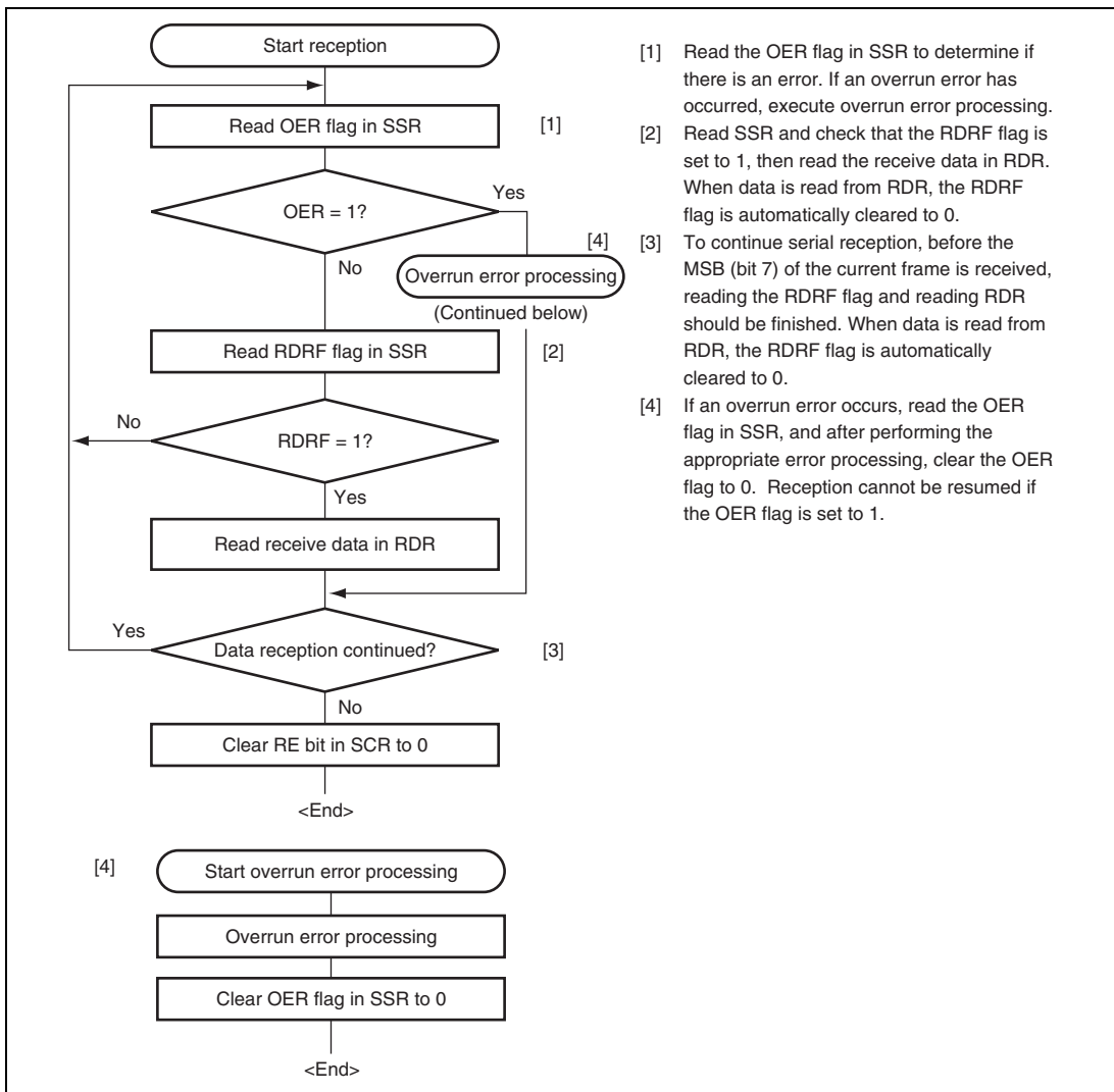
Figure 15.13 Sample Serial Reception Flowchart (Clock Synchronous Mode)
