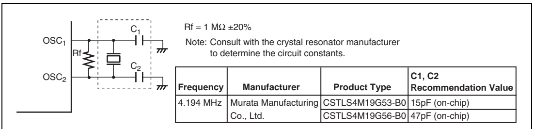
Figure 5.3 Typical Connection to Ceramic Resonator
