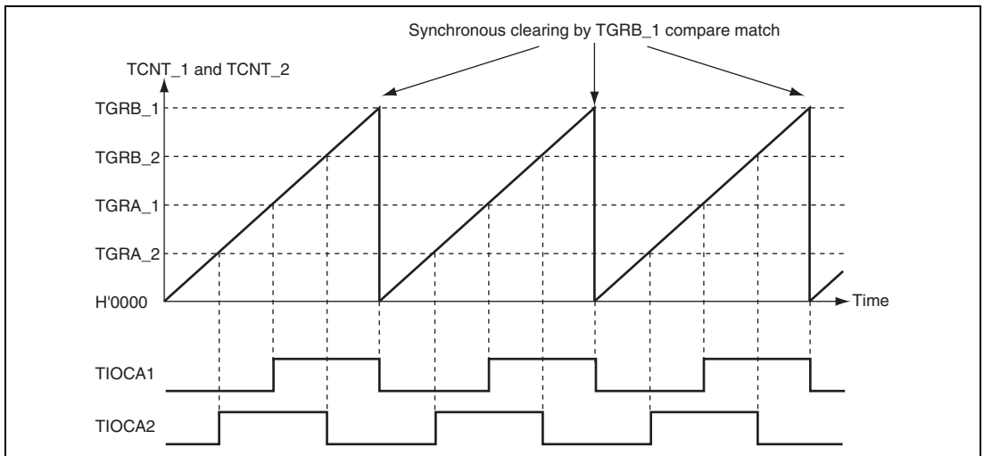
Figure 12.15 Example of Synchronous Operation
