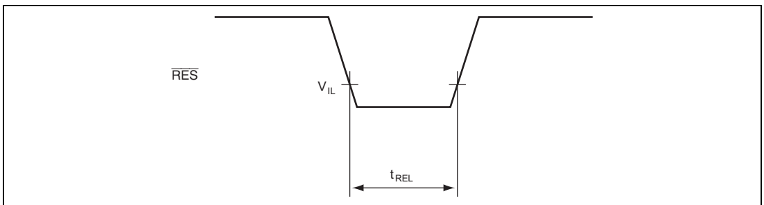
Figure 23.3 \overline{\text{RES}} Low Width Timing
