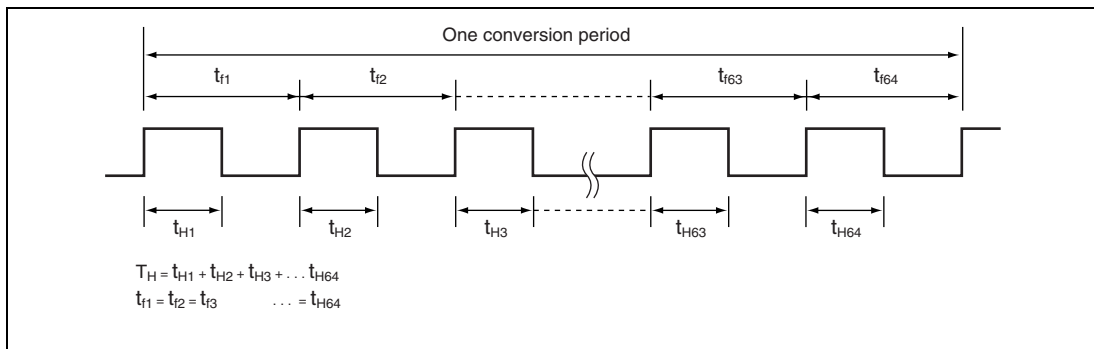
Figure 17.3 Waveform Output by PWM
