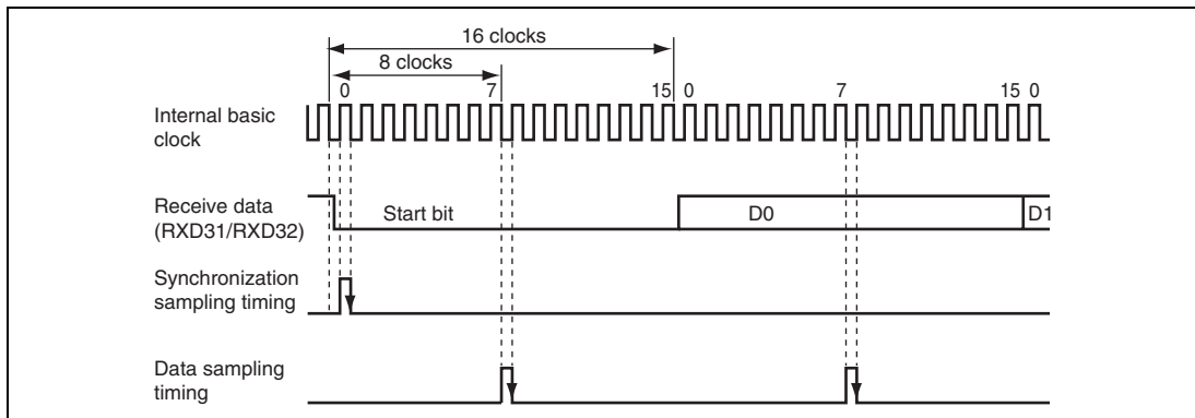
Figure 15.18 Receive Data Sampling Timing in Asynchronous Mode
