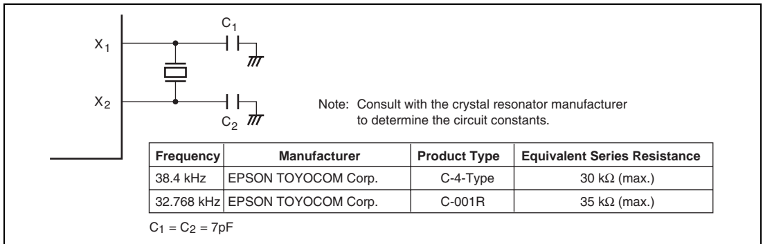
Figure 5.5 Typical Connection to 32.768-kHz/38.4-kHz Crystal Resonator
