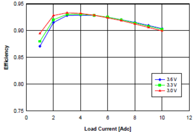
Fig. 1.5V.4: Efficiency vs. load current and input voltage for YNL05S10015 converter mounted horizontally with air flowing at a rate of 200 LFM (1 m/s) and T_a = 25 °C.
