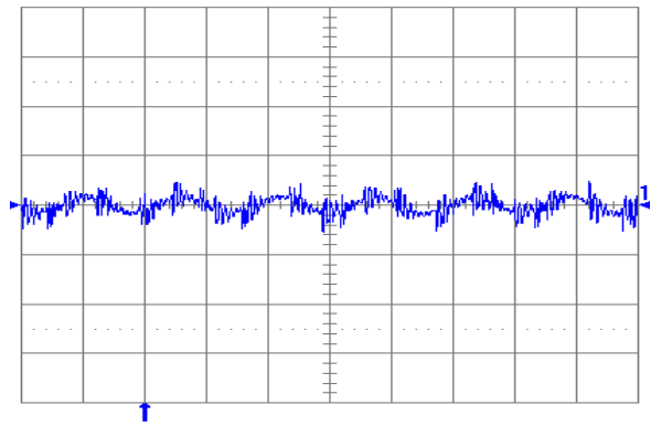
Fig. 2.0V.6: Output voltage ripple (20 mV/div.) at full rated load current into a resistive load with external capacitance 47\ \mu\text{F} ceramic + 1\ \mu\text{F} ceramic and V_{in} = 5\ \text{V} (YNL05S10020). Time scale: 2 \mu\text{s} /div.
