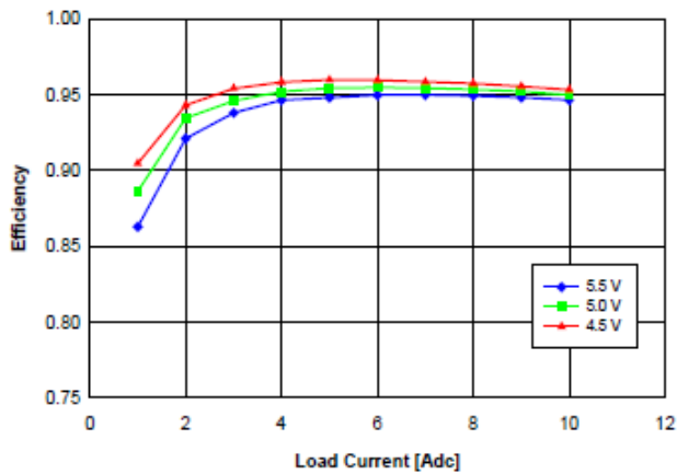
Fig. 3.3V.3: Efficiency vs. load current and input voltage for YNL05S10033 converter mounted vertically with air flowing at a rate of 200 LFM (1 m/s) and T_a = 25\text{ }^{\circ}\text{C} .
