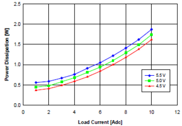
Fig. 3.3V.4: Power Loss vs. load current and input voltage for YNL05S10033 converter mounted vertically with air flowing at a rate of 200 LFM (1 m/s) and T_a = 25\text{ }^{\circ}\text{C} .
