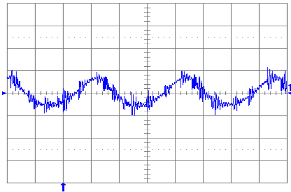
Fig. 3.3V.6: Output voltage ripple (20 mV/div.) at full rated load current into a resistive load with external capacitance 47\text{ }\mu\text{F} ceramic + 1\text{ }\mu\text{F} ceramic and V_{in} = 5\text{ V} (YNL05S10033) Time scale: 2\text{ }\mu\text{s/div} .
