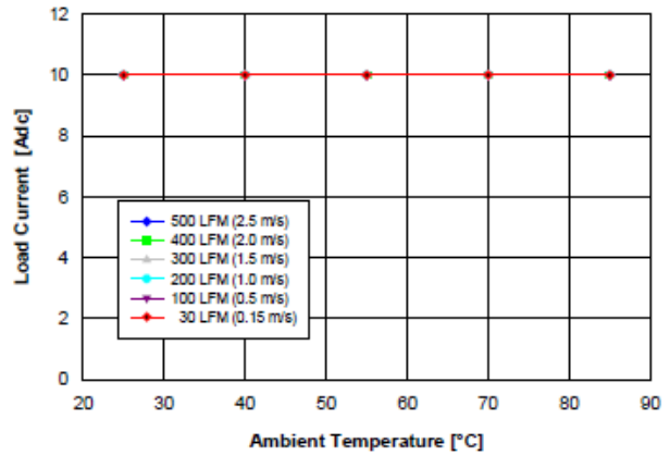
Fig. 3.3V.2: Available load current vs. ambient temperature and airflow rates for YNL05S10033 converter mounted horizontally with V_{in} = 5\text{ V} , and maximum MOSFET temperature \leq 110\text{ }^{\circ}\text{C} .
