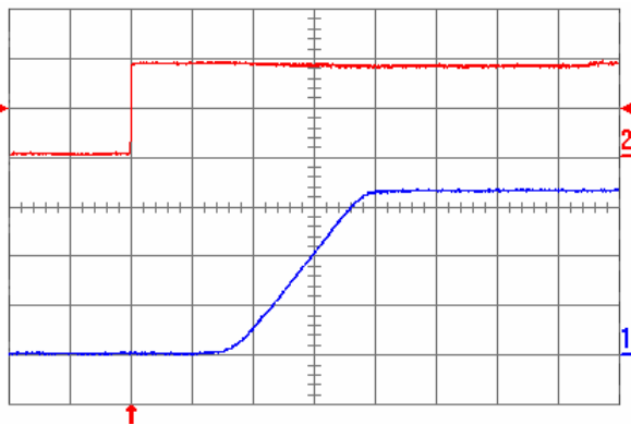
Fig. 3.3V.5: Turn-on transient (YNL05S10033) with the application of Enable signal at full rated load current (resistive) and 47\text{ }\mu\text{F} external capacitance at V_{in} = 5\text{ V} . Top trace: Enable signal (2 V/div.); Bottom trace: output voltage (1 V/div.); Time scale: 2 ms/div.
