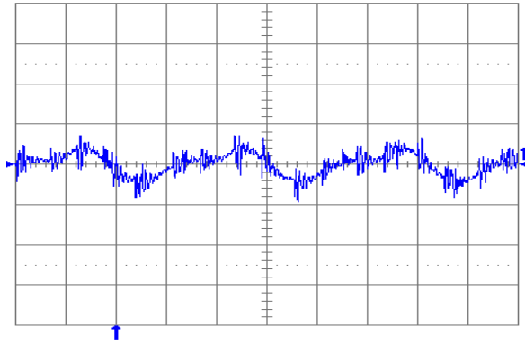
Fig. 2.5V.6: Output voltage ripple (20 mV/div.) at full rated load current into a resistive load with external capacitance 47 \mu\text{F} ceramic + 1 \mu\text{F} ceramic and V_{in} = 5\text{ V} (YNL05S10025). Time scale: 2 \mu\text{s} /div.
