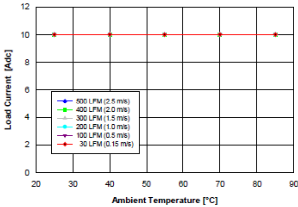
Fig. 3.3V.1: Available load current vs. ambient temperature and airflow rates for YNL05S10033 converter mounted vertically with V_{in} = 5\text{ V} , and maximum MOSFET temperature \leq 110\text{ }^{\circ}\text{C} .
