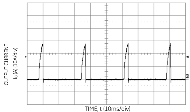
Figure 18. Output short circuit Current ( V_{in} = 5.0\text{ Vdc} , V_o = 0.75\text{ Vdc} ).
