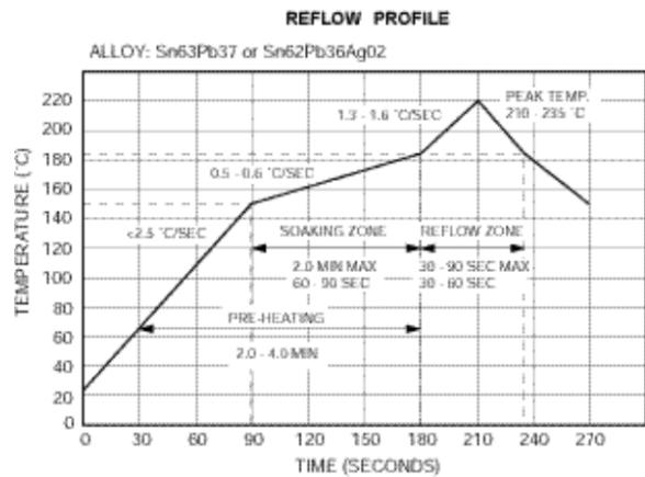
Figure 36. Reflow Profile.
