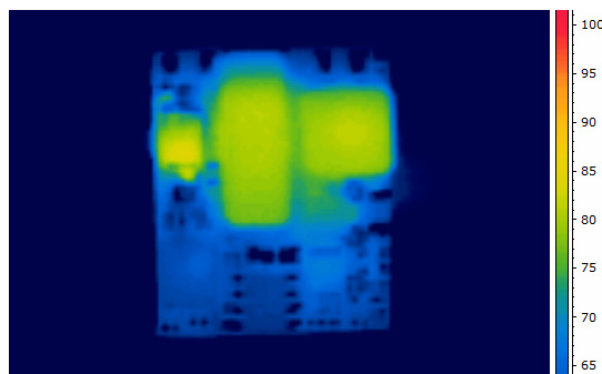
Figure 7. Thermal Image of CPZ5A48 (5A output, 25C Ambient, no airflow, Vin = 48V, T max = 85°C)
