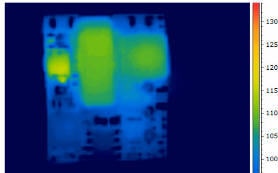
Figure 8. Thermal Image of CPZ5A48 (5A output, 70C Ambient, 200lfm airflow, Vin = 48V, T max = 115°C)
