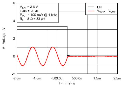
Figure 30. Shutdown Timing
