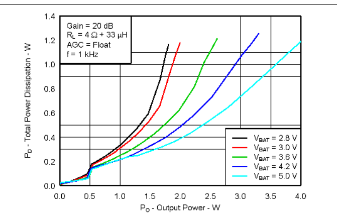
Figure 18. Total Power Dissipation vs Output Power
