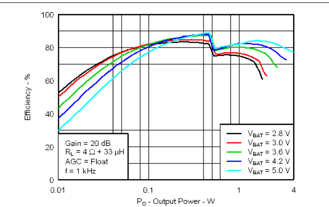
Figure 16. Total Efficiency vs Output Power
