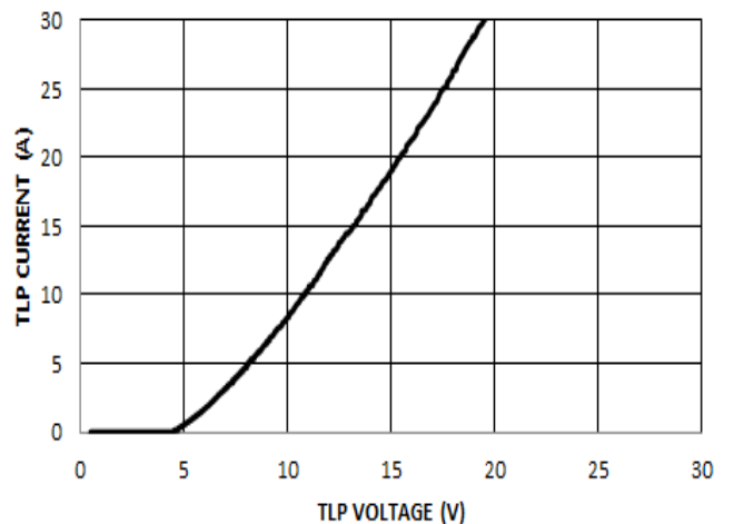
Figure 8 TLP Curve (tp=100ns)
