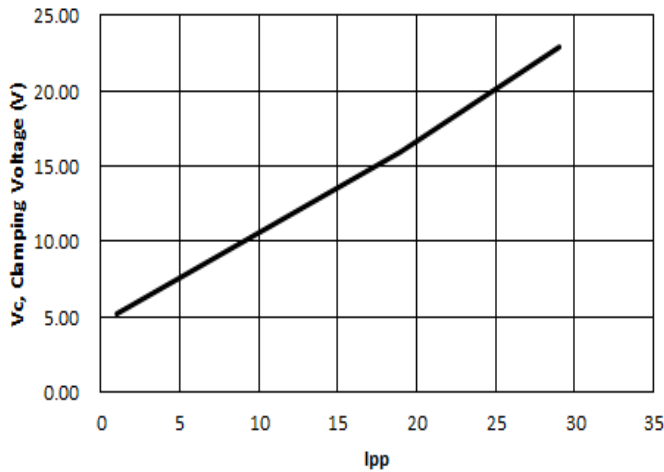
Figure 7 Clamping Voltage Characteristic (tp=8/20µs)
