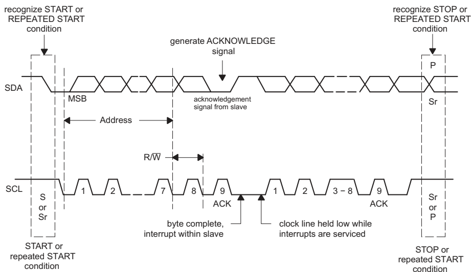
Figure 43. Bus Protocol
