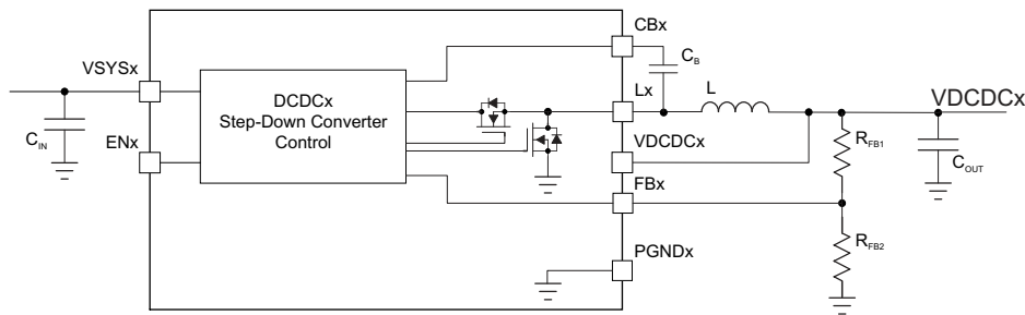
Figure 69. DC-DC Converters Circuit Drawing
