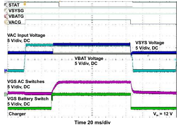
Figure 64. Adapter Input Power Up and Power Down
