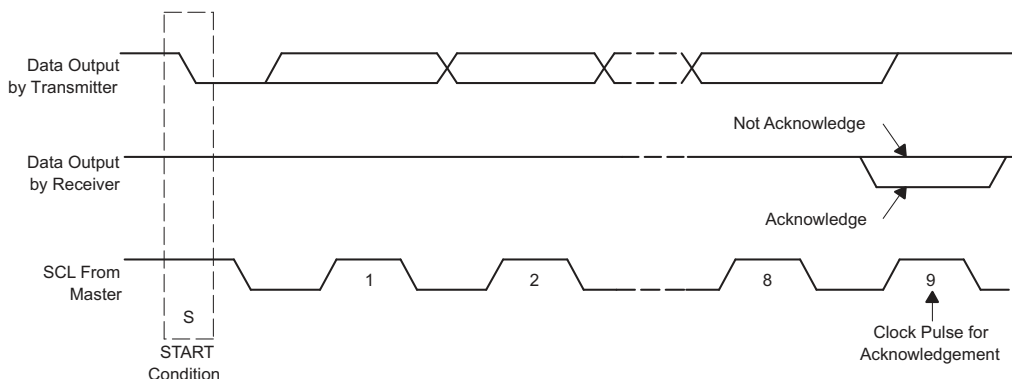
Figure 42. Acknowledge on the I 2 C-Bus
