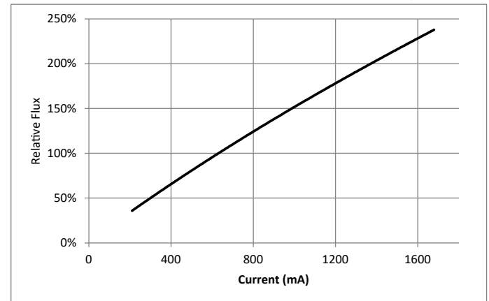
Figure 12: V13C Typical Relative Flux vs. Current ( T_c=25^\circ\text{C} )
