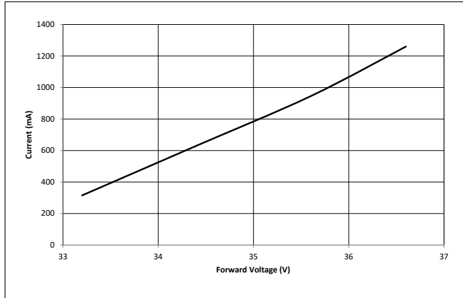
Figure 11: V13C Drive Current vs. Voltage ( T_c=25^\circ\text{C} )
