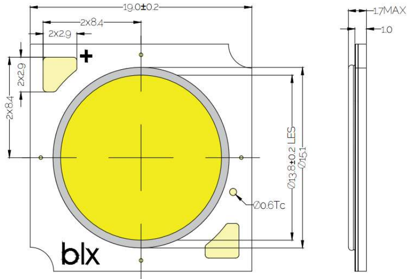
Figure 18: V13 LED Array
