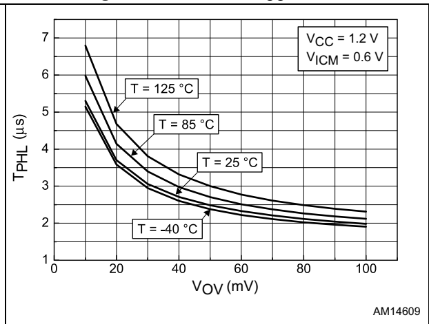
Figure 25. Propagation delay T_{PHL} vs. input signal overdrive at V_{CC} = 1.2 V
