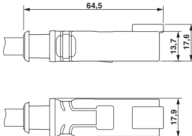
DEUTSCH DT04-2P, top view and side view
