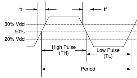
Figure 3. Output Waveform
