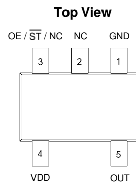
Figure 1. Pin Assignments
