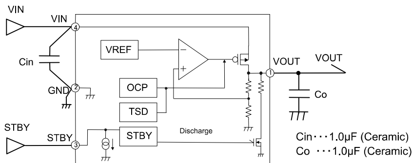
Figure 2. Block Diagrams
