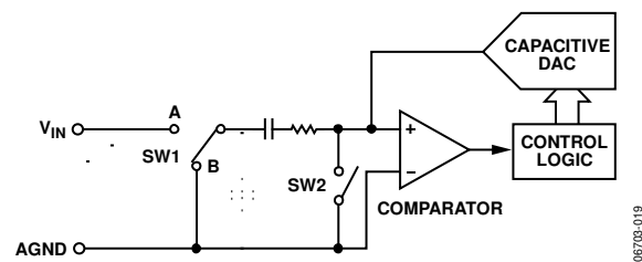
Figure 17. ADC Conversion Phase
