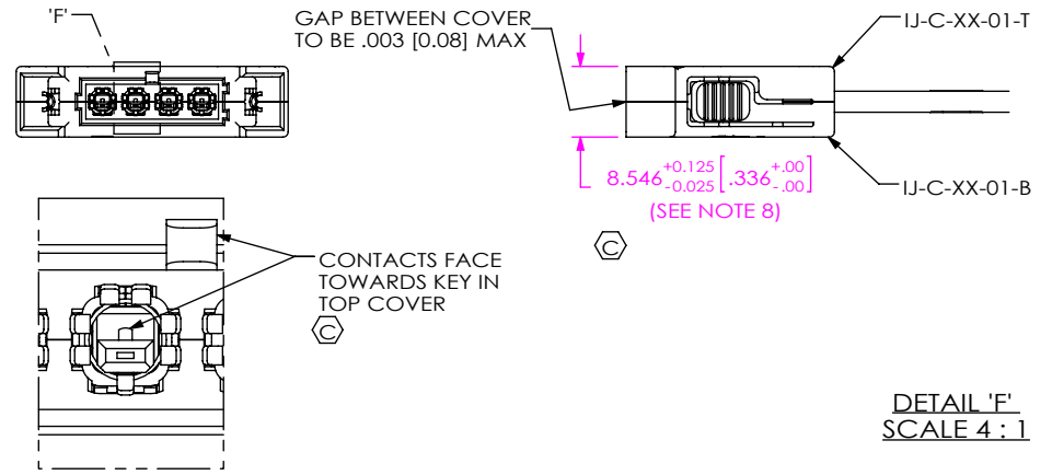
IN-PROCESS STEP 8 (THERMO WELD COVERS)
