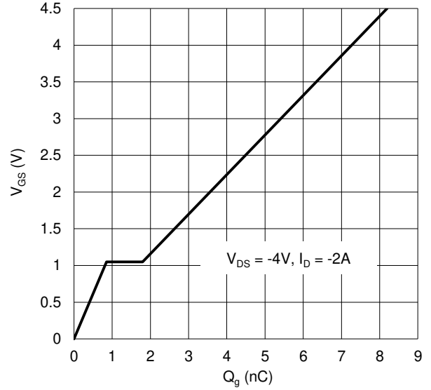
Figure 10. Gate Charge
