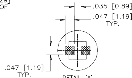
DETAIL 'A' (ENLARGED) SMT LED SOLDER PAD (SMT LED TO BE PROVIDED BY THE CUSTOMER)
