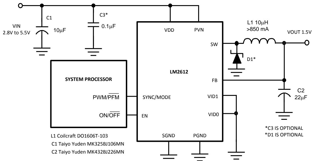
Figure 41. Typical Operating Circuit
