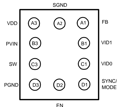
Figure 2. BOTTOM VIEW
