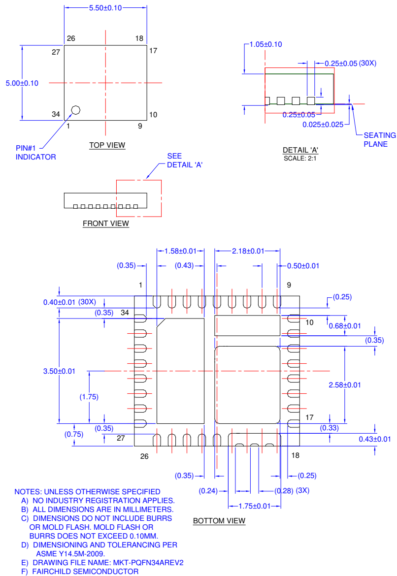
Figure 32.34-Lead, PQFN, 5.5 mm x 5.0 mm Package
