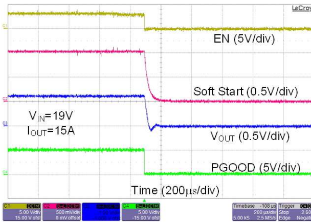
Figure 18. Shutdown Waveforms with 15 A Load Current
