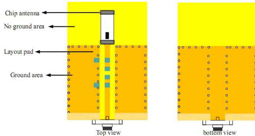
Figure shows the PCB layout highlighting the Ground and No Ground areas and trace feed line to the chip antenna.
