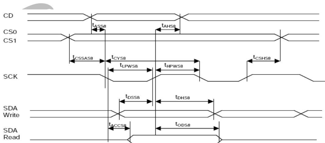
FIGURE 2 : Serial Bus Timing Characteristics (for S8)
