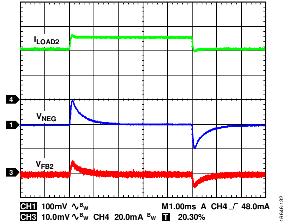
Figure 32. Inverting Regulator Load Transient, V_{IN} = 5\text{ V} Step, V_{NEG} = -15\text{ V} , I_{LOAD2} = 35\text{ mA} to 45\text{ mA} Step, f_{SW} = 2.4\text{ MHz} , T_A = 25^\circ\text{C}
