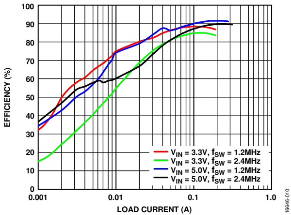
Figure 10. Efficiency vs. Load Current for Boost Regulator, V_{POS} = 15V , T_A = 25^\circ C
