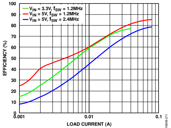
Figure 11. Efficiency vs. Load Current for Boost Regulator, V_{POS} = 35V , T_A = 25^\circ C
