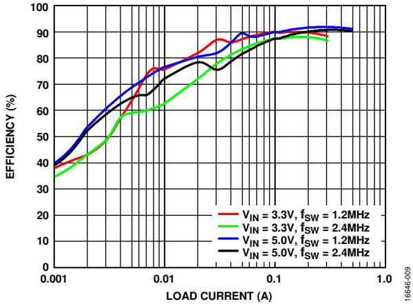
Figure 9. Efficiency vs. Load Current for Boost Regulator, V_{POS} = 9V , T_A = 25^\circ C
