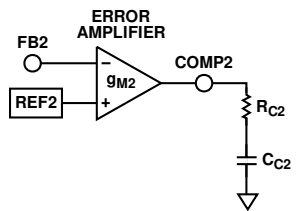
Figure 45. Compensation Component
