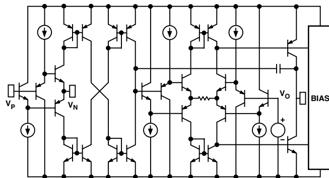
Figure 4. Simplified Schematic
