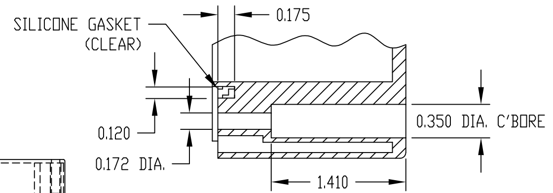
DETAIL "C"
