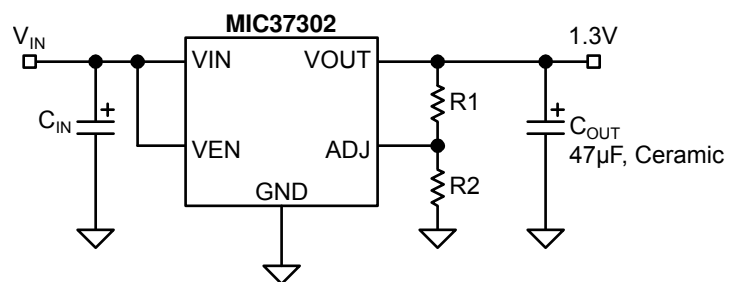
Adjustable Regulator
