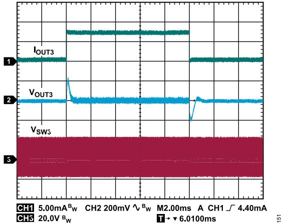
Figure 59. Inverting Regulator Load Transient Response, V_{VINP} = 24\text{ V} , V_{OUT1} = 24\text{ V} , I_{OUT1} = 0\text{ mA} , V_{OUT2} = 5\text{ V} , I_{OUT2} = 0\text{ mA} , V_{OUT3} = -15\text{ V} , I_{OUT3} = -0.3\text{ mA} to -7\text{ mA} Step, T_A = 25^\circ\text{C}
