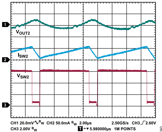
Figure 43. Buck Regulator Continuous Conduction Mode Operation Showing Inductor Current I_{SW2} , Switch Node Voltage, and Output Ripple, T_A = 25^\circ\text{C} , V_{OUT1} = 6\text{ V} , V_{OUT2} = 5\text{ V} , I_{OUT2} = 30\text{ mA}
