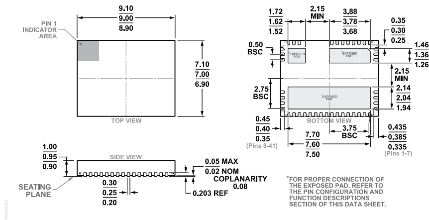
Figure 91. 41-Lead Lead Frame Chip Scale Package [LFCSP] 9 mm x 7 mm Body and 0.95 mm Package Height (CP-41-1) Dimensions shown in millimeters
