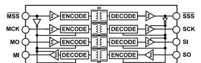
Figure 79. iCoupler Gating
