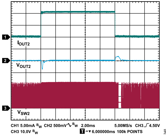
Figure 48. Buck Regulator Load Transient Response, V_{VINP} = 24\text{ V} , V_{OUT1} = 24\text{ V} , V_{OUT2} = 5\text{ V} , I_{OUT2} = 0.3\text{ mA} to 11 mA Step, T_A = 25^\circ\text{C}
