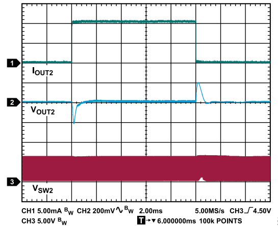
Figure 51. Buck Regulator Load Transient Response, V_{VINP} = 24\text{ V} , V_{OUT1} = 6\text{ V} , V_{OUT2} = 5\text{ V} , I_{OUT2} = 0.3\text{ mA} to 11 mA Step, T_A = 25^\circ\text{C}
