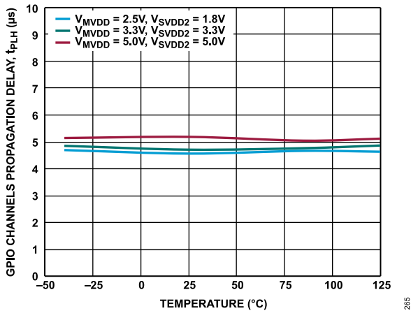
Figure 72. GPIO Channels Propagation Delay ( t_{PLH} ) vs. Temperature at Various Supply Voltages
