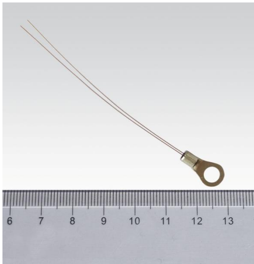
Figure 1.1. The physical photo of ATH10KL2D
