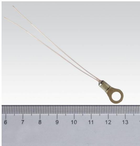
Figure 1.2. The physical photo of ATH10KL2DT70S
