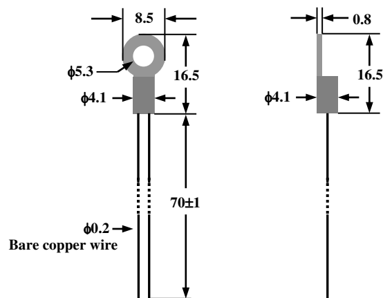
Figure 2. The Front and Side Views of ATH10KL2D
