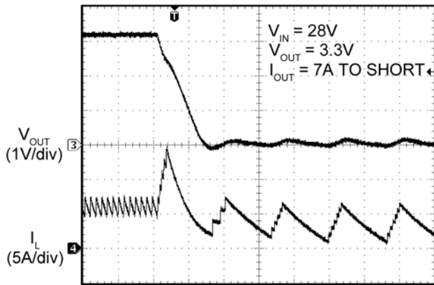
Short Circuit
