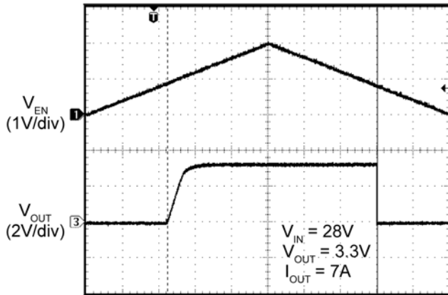
Enable Thresholds
