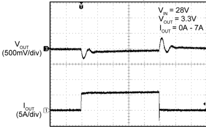
Transient Response
