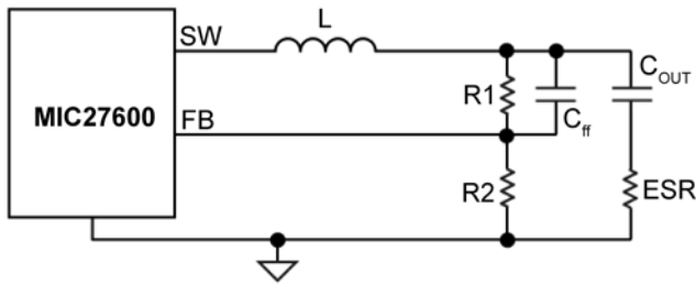
Figure 5b. Inadequate Ripple at FB
