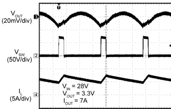
Switching Waveforms; I_{OUT} = 7A
