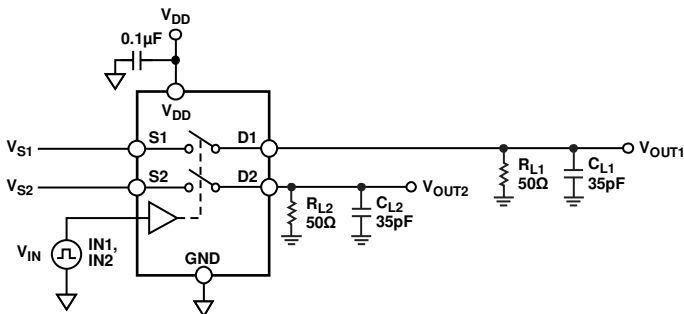
Figure 21. Break-Before-Make Time Delay, t_{BBM} (ADG823 only)
