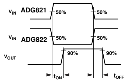
Figure 20. Switching Times
