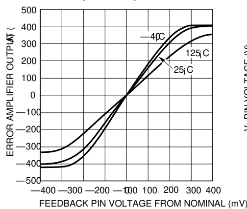
Error Amplifier Output Current
