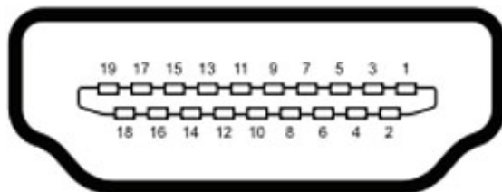
Figure 2.7 HDMI connector
