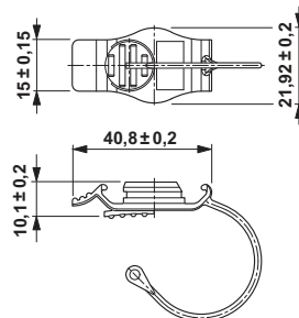
Dimensioned drawing
