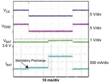
Figure 10-8. Charger ON/OFF Using \overline{\text{CE}}
