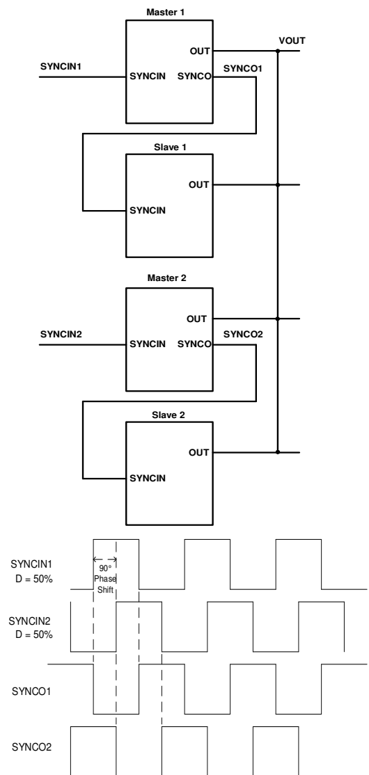
Figure 8: Four-Phase Configuration
