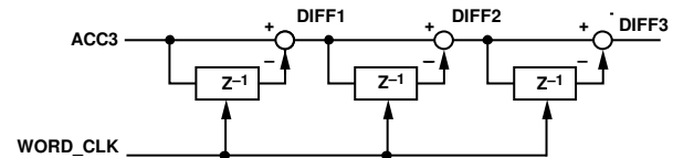
Figure 26. Differentiator
