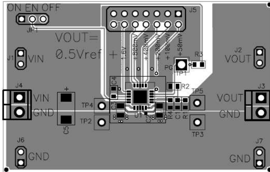
Figure 3. Assembly Layer
