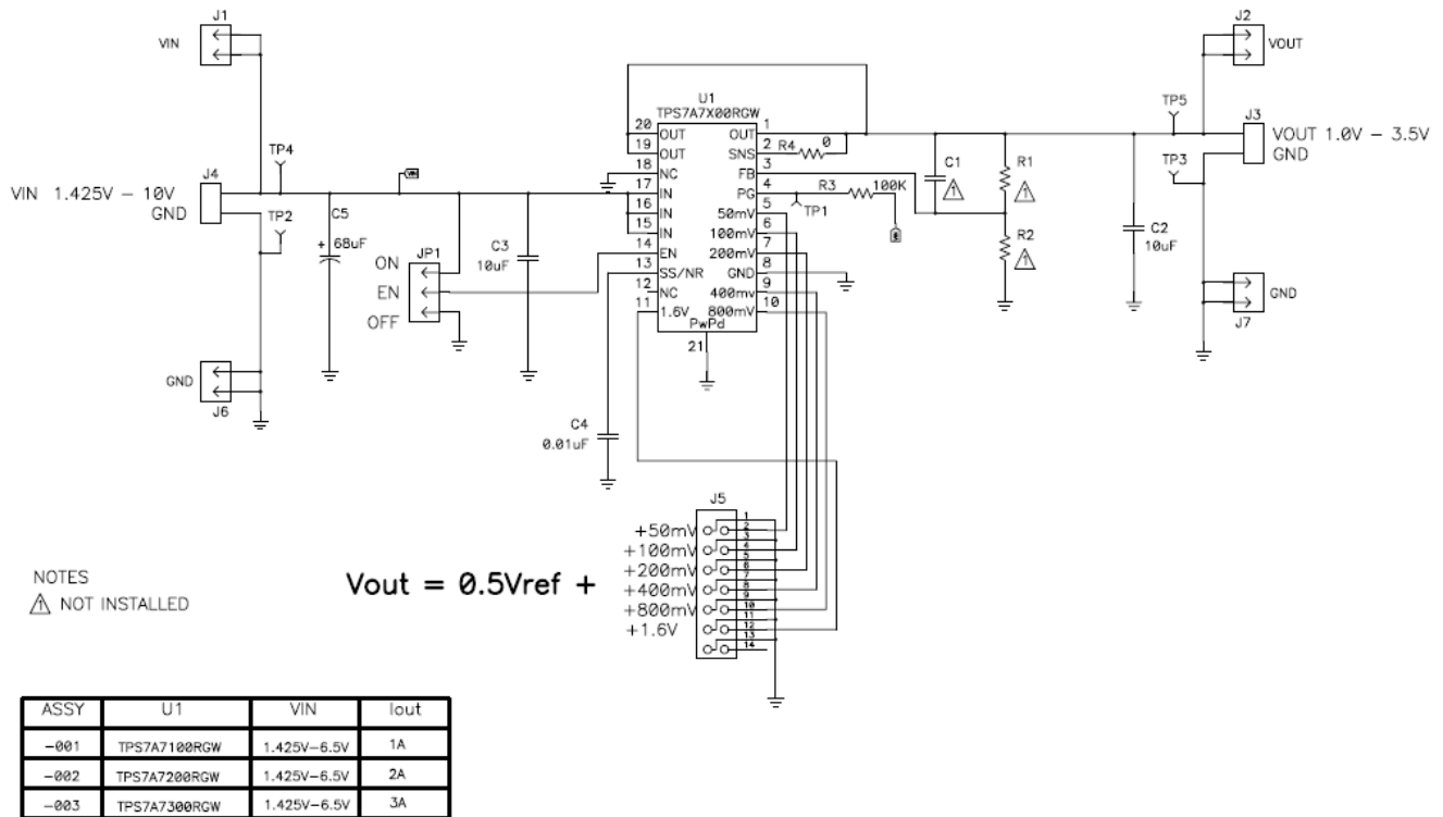
Figure 6. TPS7A7x00EVM-718 Schematic
