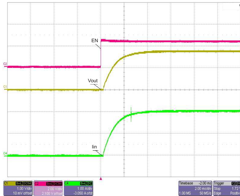
Figure 1. Turnon Sequence
