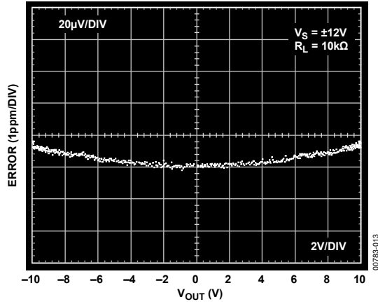
Figure 14. Gain Nonlinearity; V_S = \pm 12\text{ V} , R_L = 10\text{ k}\Omega
