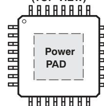
VFP PACKAGE (TOP VIEW)
