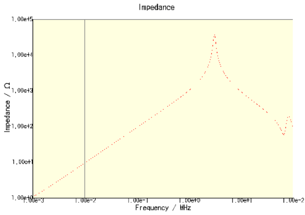
CLF6045T-151M-CA
