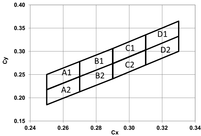
Figure 2: Chromaticity Diagram
