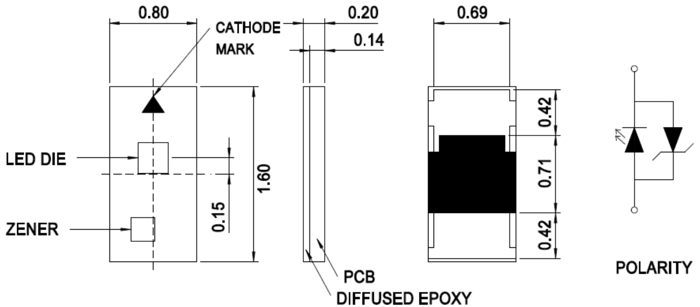
Figure 1: Package Dimensions
