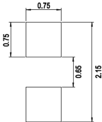
Figure 8: Recommended Soldering Land Pattern
