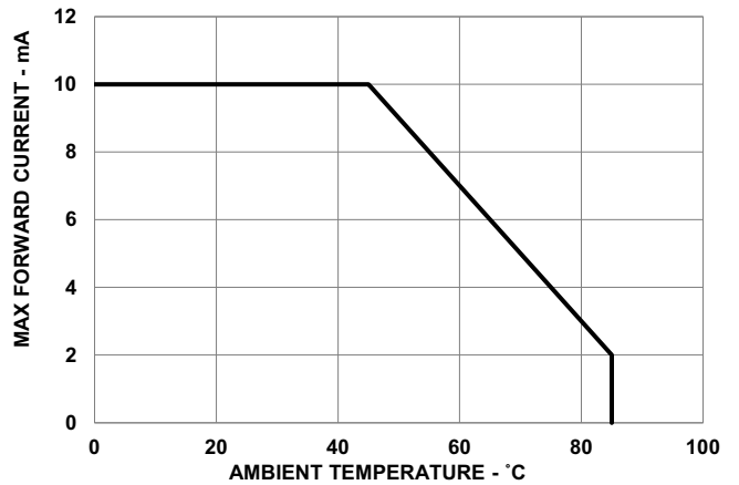
Figure 7: Derating Curve
