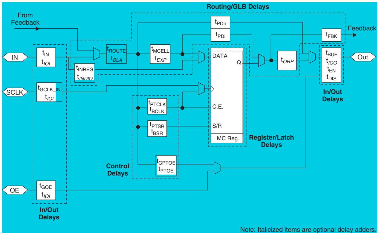
Figure 11. LA-ispMACH 4000V/Z Automotive Timing Model
