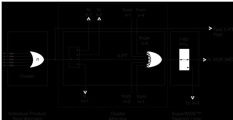
Figure 4. Macrocell Slice
