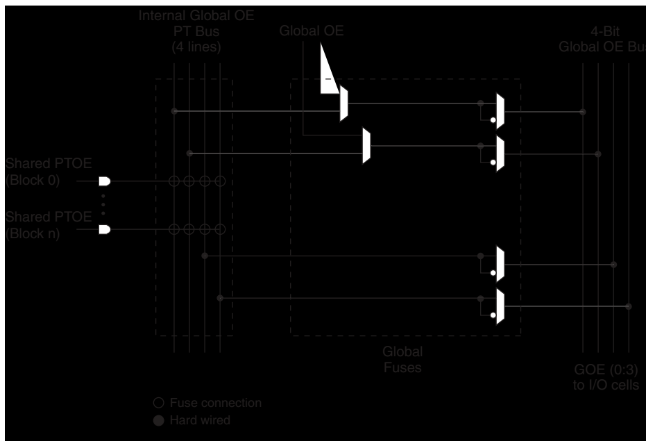
Figure 10. Global OE Generation for LA-ispMACH 4032V/Z
