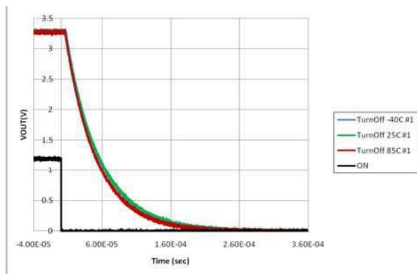
Figure 22. Turn-Off Response (FPF1207 = No Output Pull-Down Resistor) (V IN =3.3V, C IN =1μF, C OUT =0.1μF, R L =500Ω)
