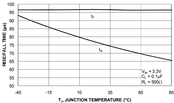
Figure 18. V OUT Rise and Fall Time vs. Temperature at R L =500Ω
